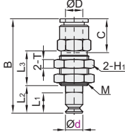
Pad Diameter Ø6,Ø8
