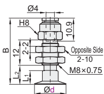
Fixed Type, Vacuum Port on Top J-WEU61/62
