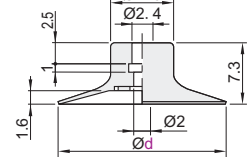
Pad Diameter Ø20
