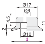
Pad Diameter Ø25
