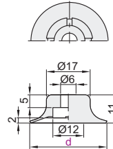
Pad Diameter Ø30
