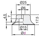
Pad Diameter \varnothing 40
