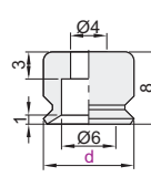
Pad Diameter Ø10
