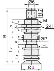
Pad Diameter Ø20~40
