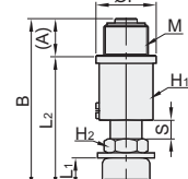
Pad Diameter \varnothing 15 \sim 30
