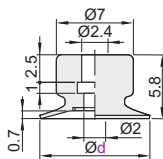
Pad Diameter Ø10
