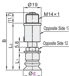
Pad Diameter Ø20~40
