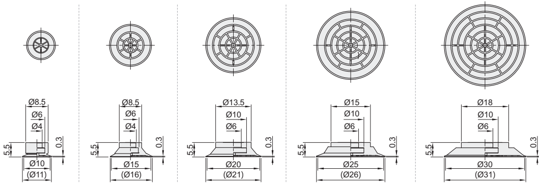
Pad Diameter Ø10
