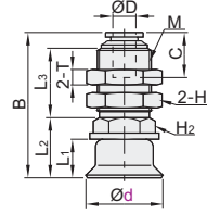
Pad Diameter Ø15~30
