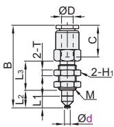
Pad Diameter Ø4
