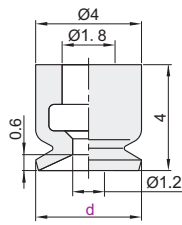
Pad Diameter Ø4
