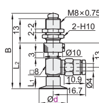
Spring Type, Vacuum Port on Side J-WEU71/72
