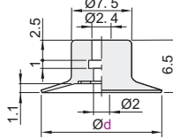
Pad Diameter Ø15
