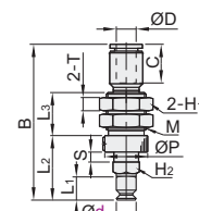
Pad Diameter Ø6,Ø8
