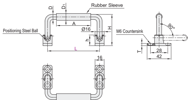
Countersink XAN01
