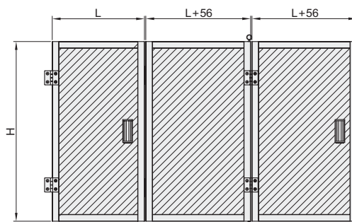
Opening dimension of door frame
