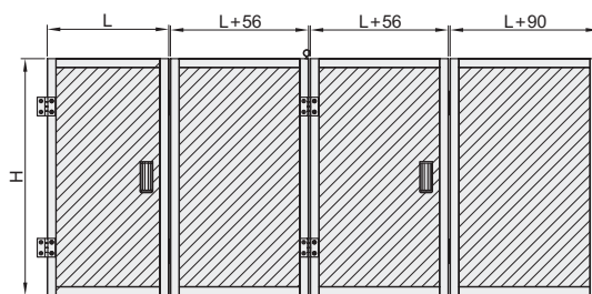
Opening dimension of door frame
